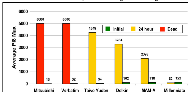
Figure 3-23 PI8 Max Average by Manufacturer Including Dead Discs
